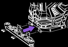
Install Squeegee (x4 bolts)
